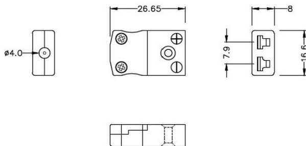
Miniature in-line Plug (dimensions in mm)
