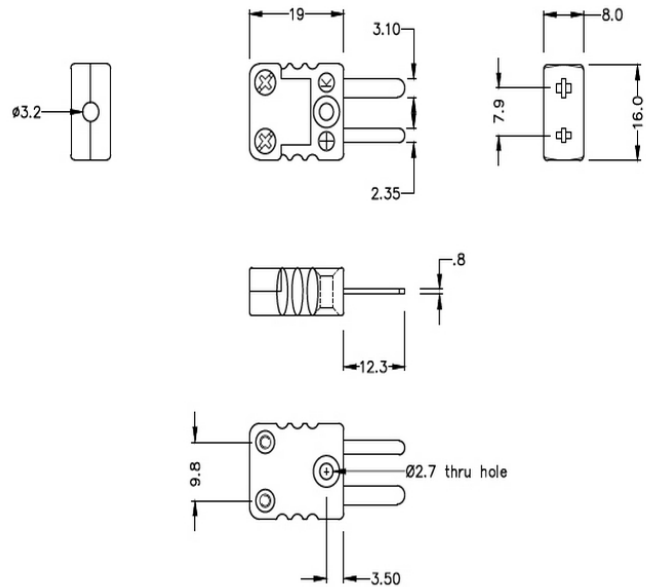
Miniature Hi-Temp Plastic in-line Plug - HTP (dimensions in mm)
